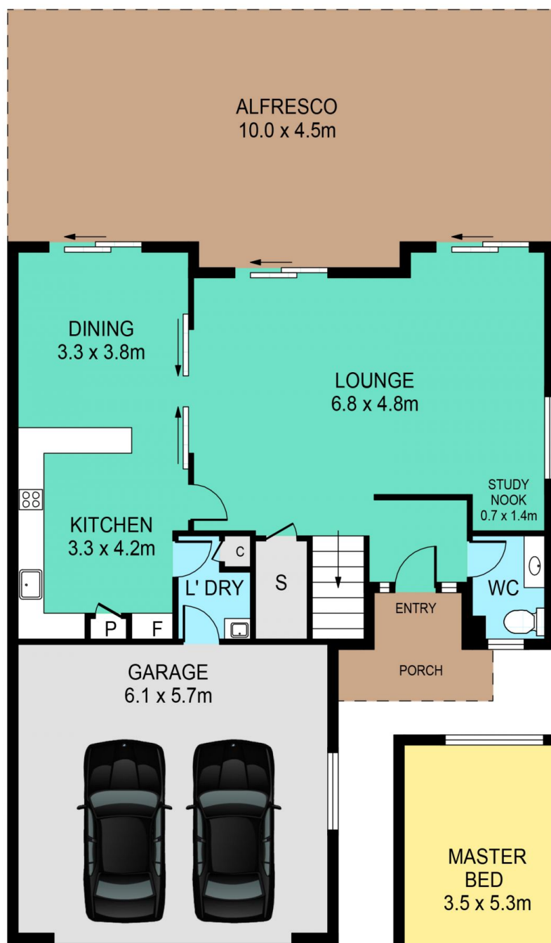
GROUND FLOOR
