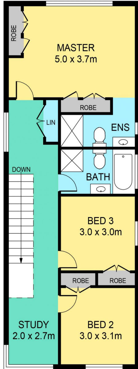
FIRST FLOOR
