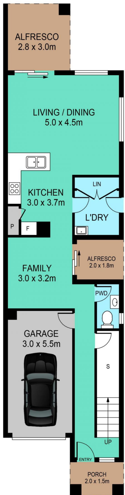
GROUND FLOOR
