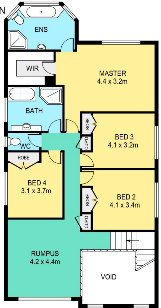
FIRST FLOOR
