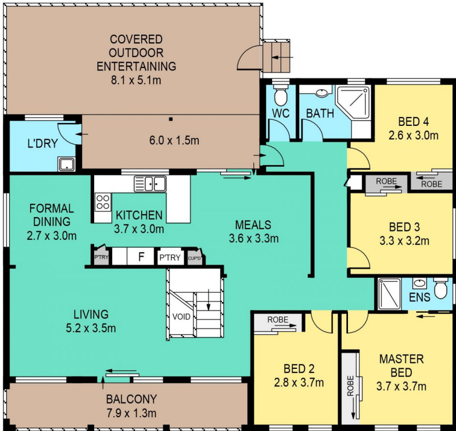
UPPER LEVEL
