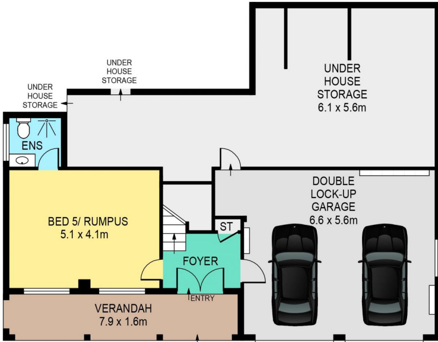
GROUND LEVEL
