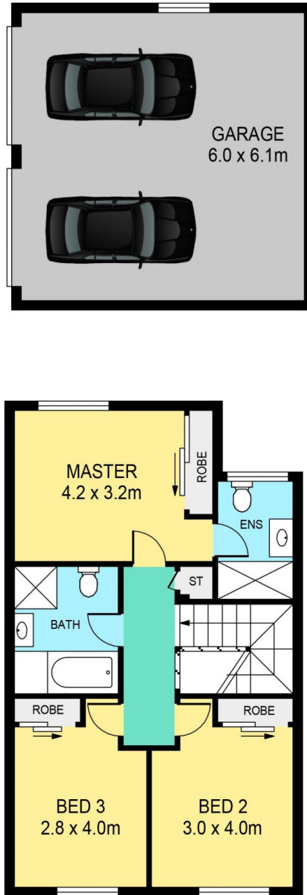
FIRST FLOOR
