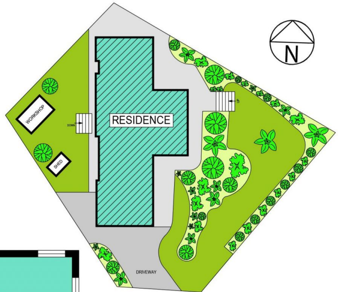
SITE PLAN
